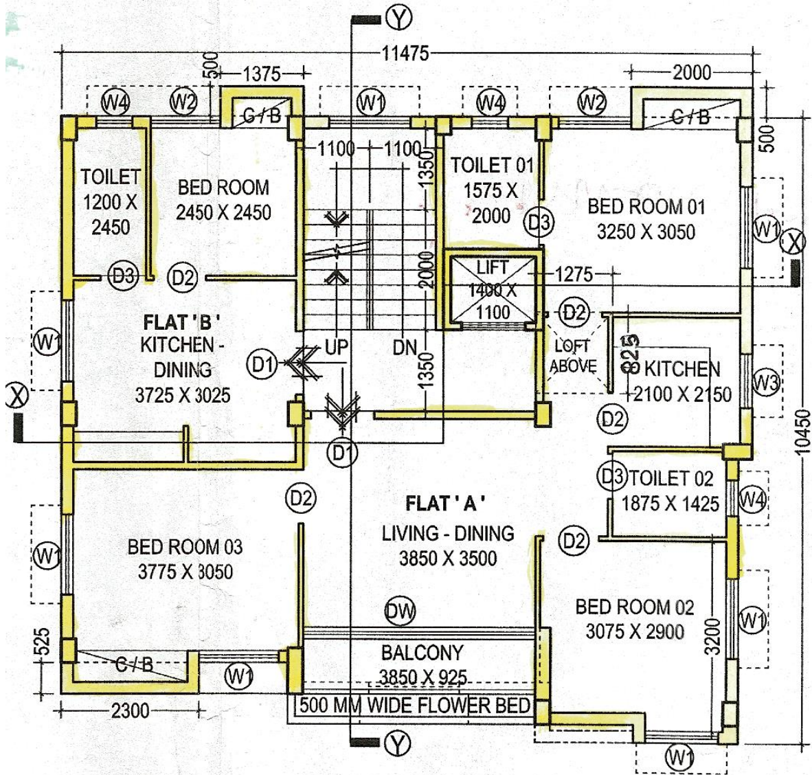
2 nd FLOOR PLAN SCALE : 1:100
