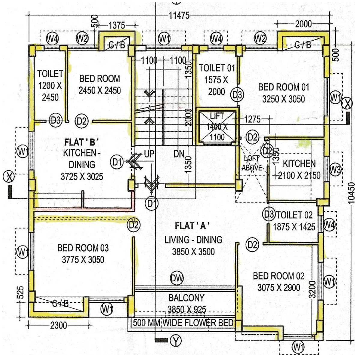
3 rd [ THIRD ] FLOOR PLAN . SCALE : 1:100
